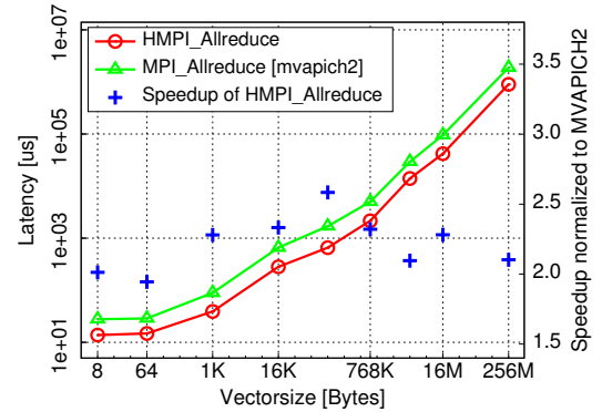
Figure 22: Performance comparison between HMPI's Allreduce and MVAPICH2 on 8-node Opteron 6100 running on 256 cores
