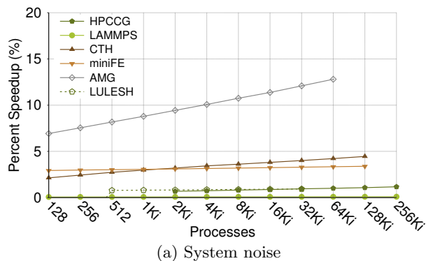
Figure 4: Impact of Cray's OS core specialization on the Volta cluster.
