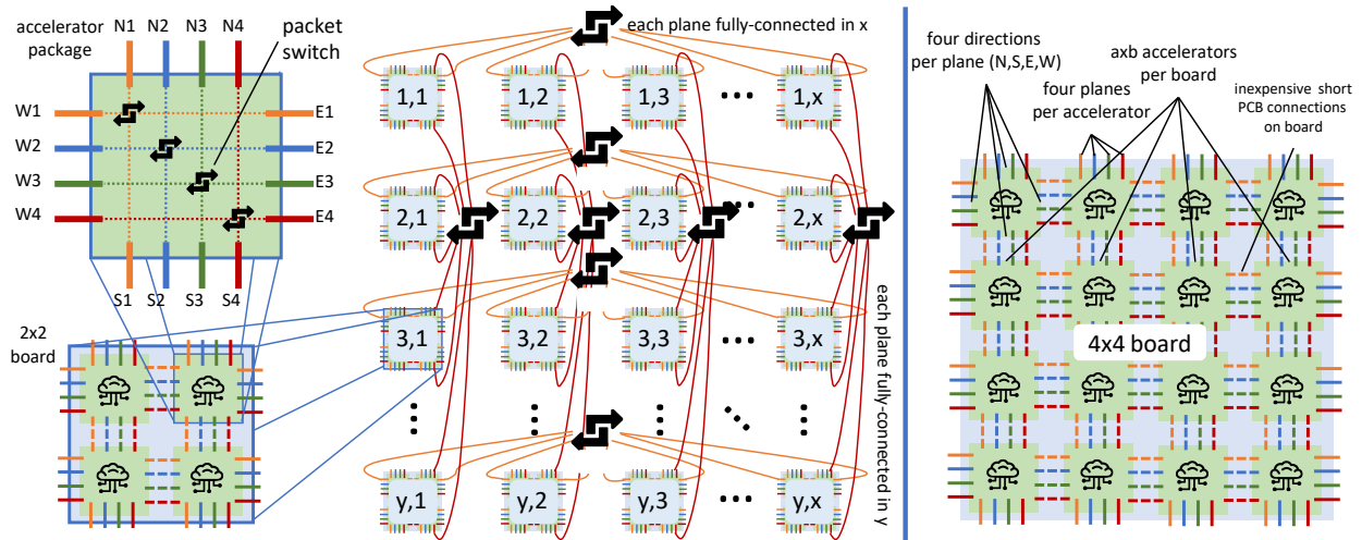
Fig. 3: HammingMesh structure: left x \times y Hx2Mesh, right Hx4Mesh board, both with four planes.
