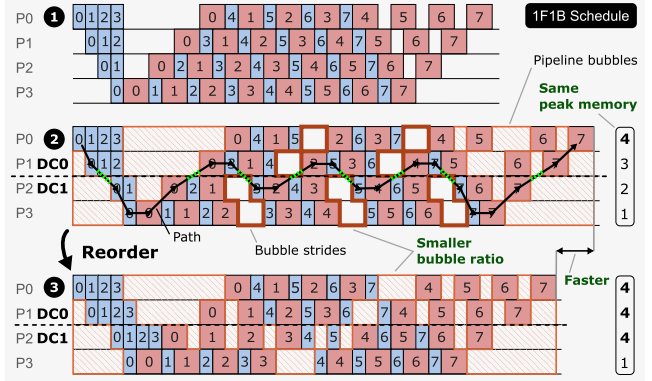
Figure 6: 1 Original 1F1B schedule. 2 1F1B schedule with Cross-DC PP communication which leads to bubble strides . A Path is depicted ( \rightarrow ) including cross-DC boundary crossings ( \leftrightarrow ). 3 The schedule after reordering is more efficient while maintaining the same peak memory. More microbatches or memory budget can help to further reduce runtime.
