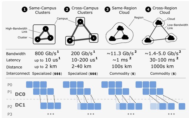
Figure 2: Cross-DC infrastructure setup types and their impact on the PP communication at DC boundaries.
