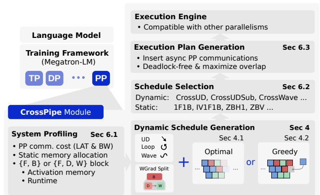
Figure 10: Components of the CrossPipe module.
